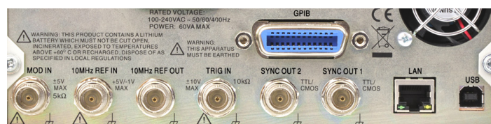
Rear panel mounting of digital interfaces and I/O connectors.
