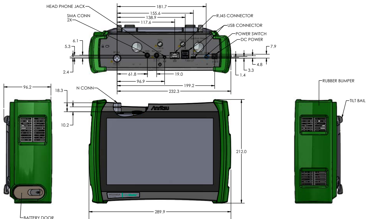
MS2085A/89A
