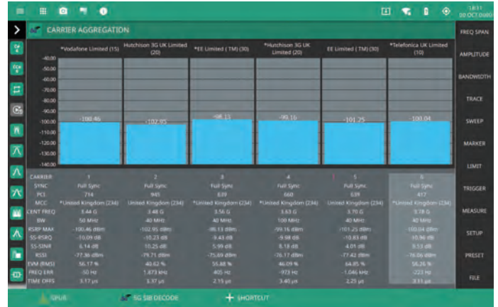
Modulation Measurement Options Perform Modulation Analysis on LTE and 5G Base Station Wave Signals
