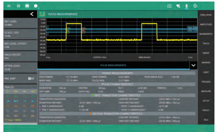
The MS27201A Pulse Analyzer Option Automates the Capture and Display of Pulsed Signals, Providing a Comprehensive Readout of All Standard Measurements
