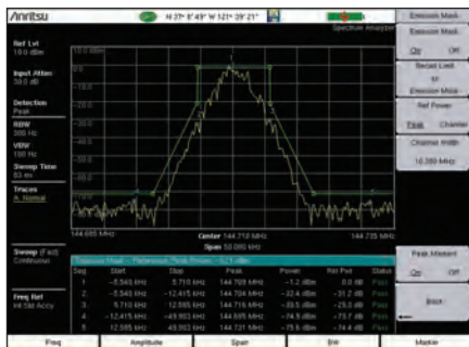
The Spectrum Analyzer Made in the LMR Master Offers Automated Measurements Including Occupied Bandwidth, Adjacent Channel Power, and Emission Mask, as Shown Above. The Mask can be Quickly Created Using the Standard Limit Line Editor. The Emission Mask Measurement Function Automatically Moves the Trace to Match the Peak of a Modulated Signal to Conform to Common Mask Standards.
