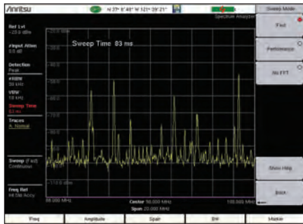
The Spectrum Analyzer Made in the LMR Master Offers Fast Sweep Speeds for Interference Hunting Intermittent Signals
