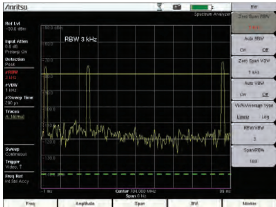
10 ms Zero Span Time
